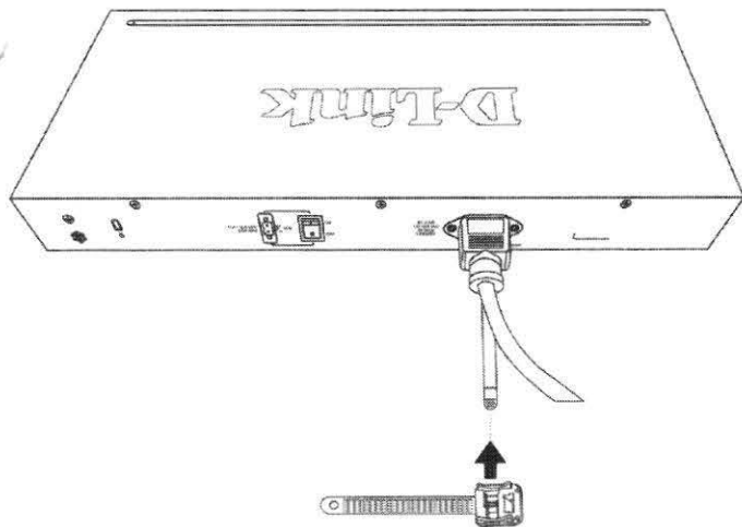
Attach the retainer to the tie wrap
